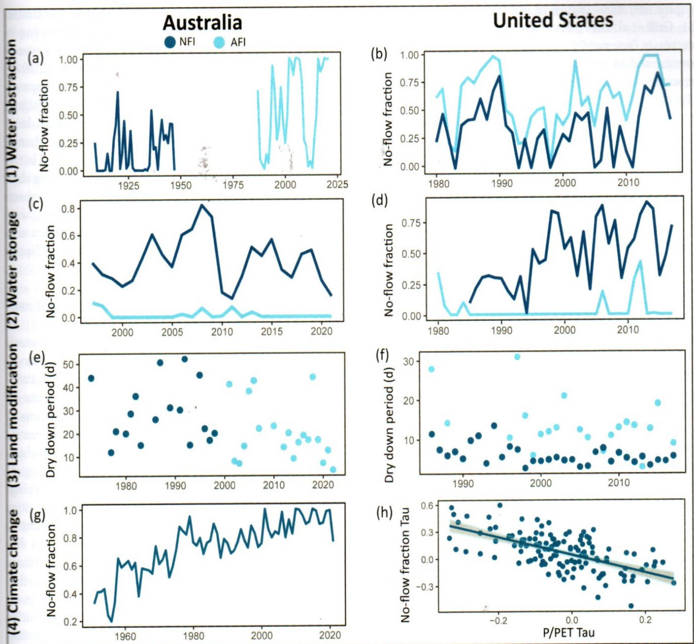
Figure 1. Differences in hydrological signatures between natural (NFI) and anthropogenic (AFI) flow intermittence for four drivers of AFI in Australia (a, c, e, g) and the United States (b, d, f, h), as is summarized in supplemental material S1. No-flow fraction is the proportion of zero-flow days in a year, whereas dry-down period is defined as the number of days from peak flow to zero flow. Panel (h) shows the relationship between the strength of the trend (tau values of Mann-Kendall trend test) in no-flow fraction over time and the strength of the trend in climatic aridity (the ratio of annual precipitation, P , to potential evapotranspiration, PET ) over time in the United States. The results with negative P:PET tau correspond to climate conditions, which have become drier.
